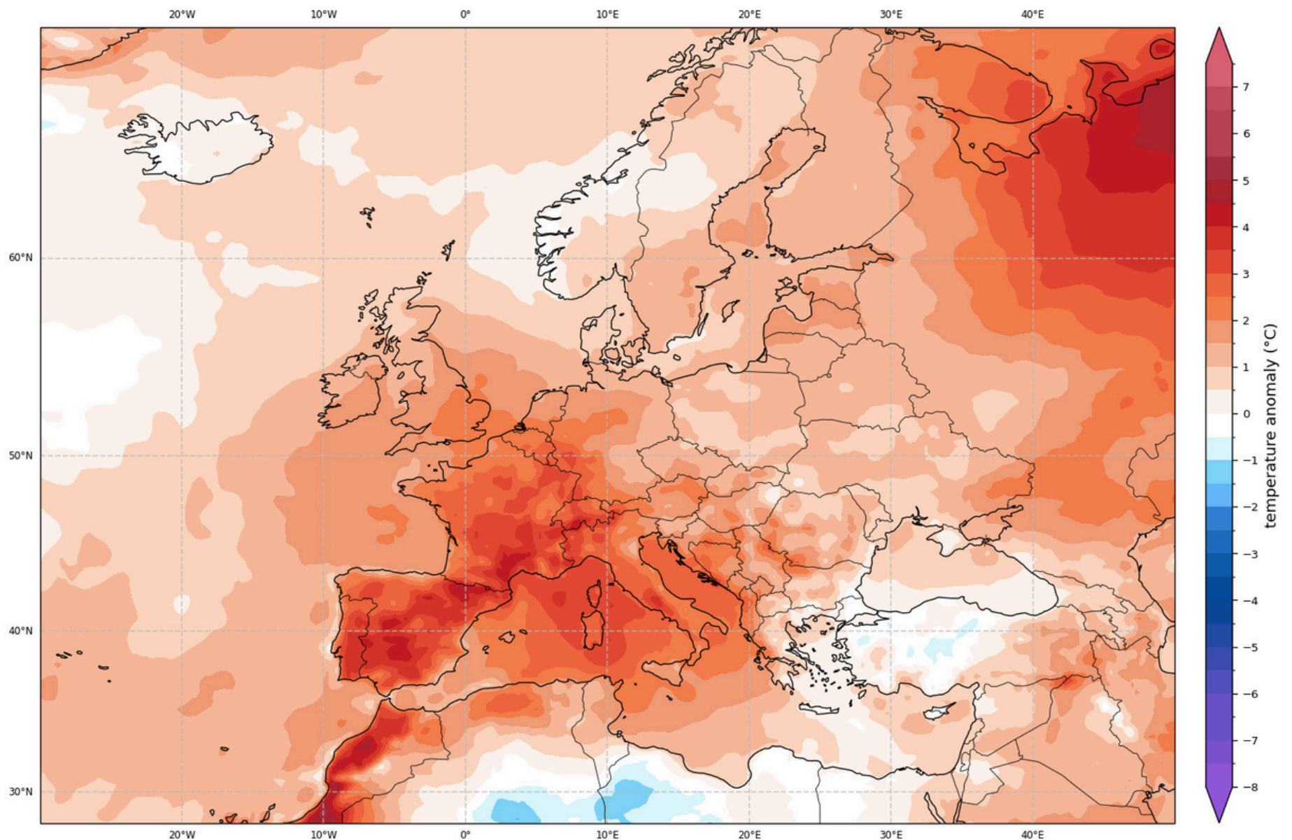
2 m temperature anomaly for September 2026 (1991-2020 climatology)
